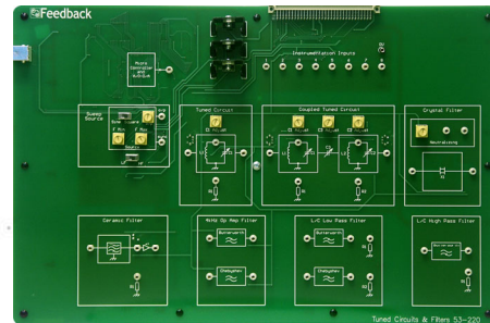
Tuned Circuits & Filters
