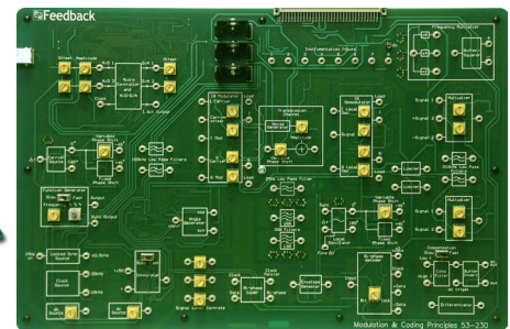
Modulation & Coding
