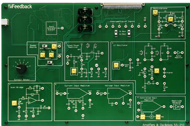
Workboard showing circuit block diagrams
