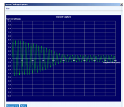
Motor in-rush current display
