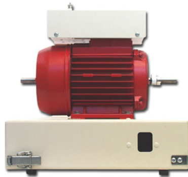
The Three phase Induction Motor 64-501 is supplied as part of the Core System
