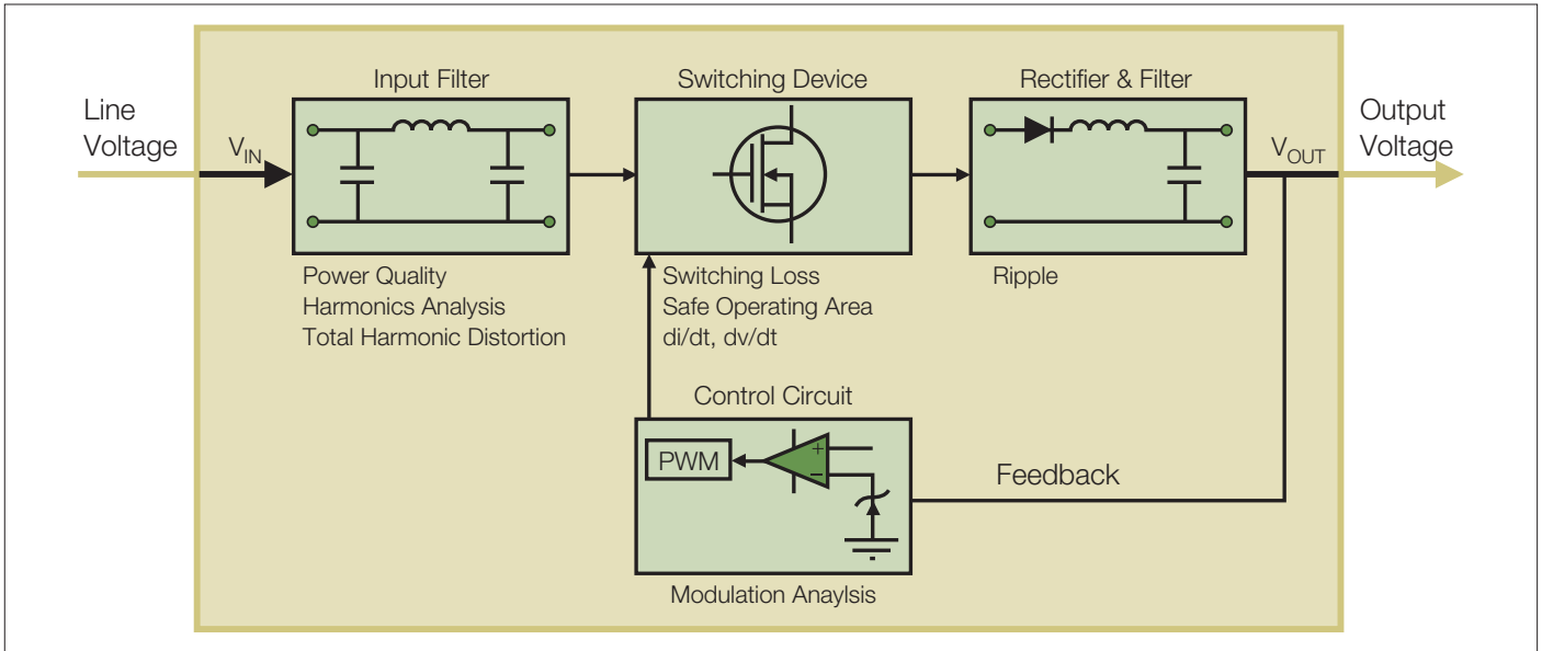
Figure 1. SMPS Components that are Characterized with DPOxPWR Power Analysis Software.
