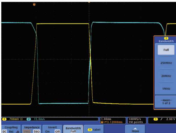
Figure 10. Bandwidth Limiting Filters Available on an MSO/DPO4000 Series Oscilloscope with a TDP1000 Attached.
